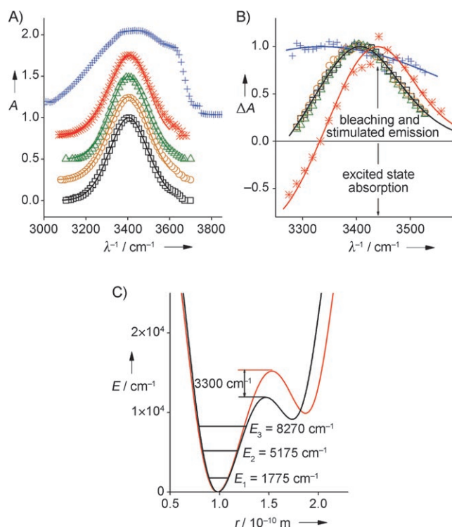
Figure 2. A) Normalized IR absorption spectra of surface water in a 1 nm sample in a low hydration state (+), confined water in fully hydrated 50 nm ( \Delta ), 13 nm ( \circ ), and 1 nm ( \square ) samples, and bulk water (*) in the OH stretching region. For clarity, the normalized spectra are offset by 0.2 absorbance units with respect to each other. The solid lines for water and nanoconfined water are obtained from a modified Lippincott-Schroeder [21,22] model. B) Normalized initial transient spectra of bulk, confined, and surface water; symbols as in (A). The solid lines for water (in red) and nanoconfined water (in black) are obtained from the same Lippincott-Schroeder model as for (A). The line for surface water is drawn to guide the eye. C) Potential ( E ) of a O-H...O system as described by the modified Lippincott-Schroeder model used in (A) and (B) for bulk (red) and confined (black) water. r is the O-H distance; the other parameters of the model are given in Table S4 in the Supporting Information, and the energy levels are given for nanoconfined water.
